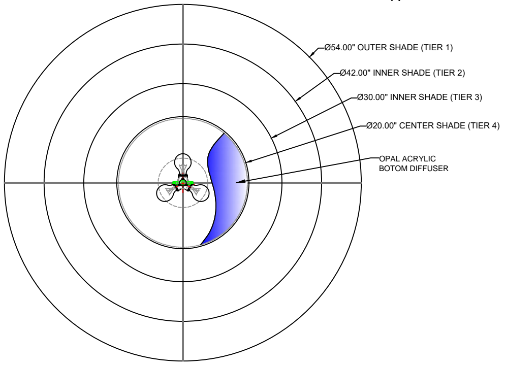
VIEW "A"-"A"
