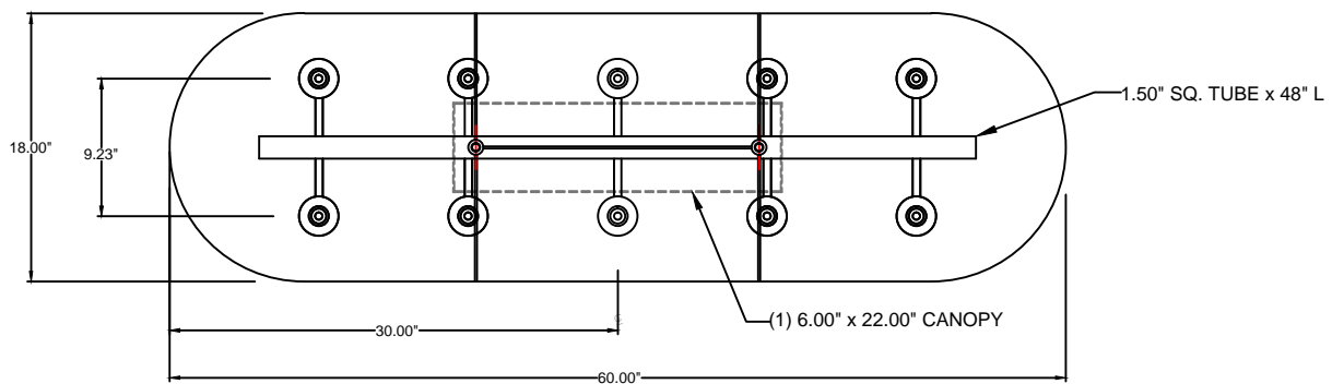
"BOTTOM VIEW "
