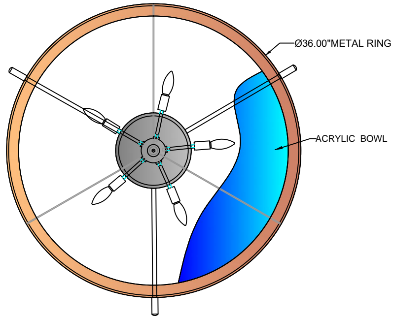
BOTTOM VIEW
