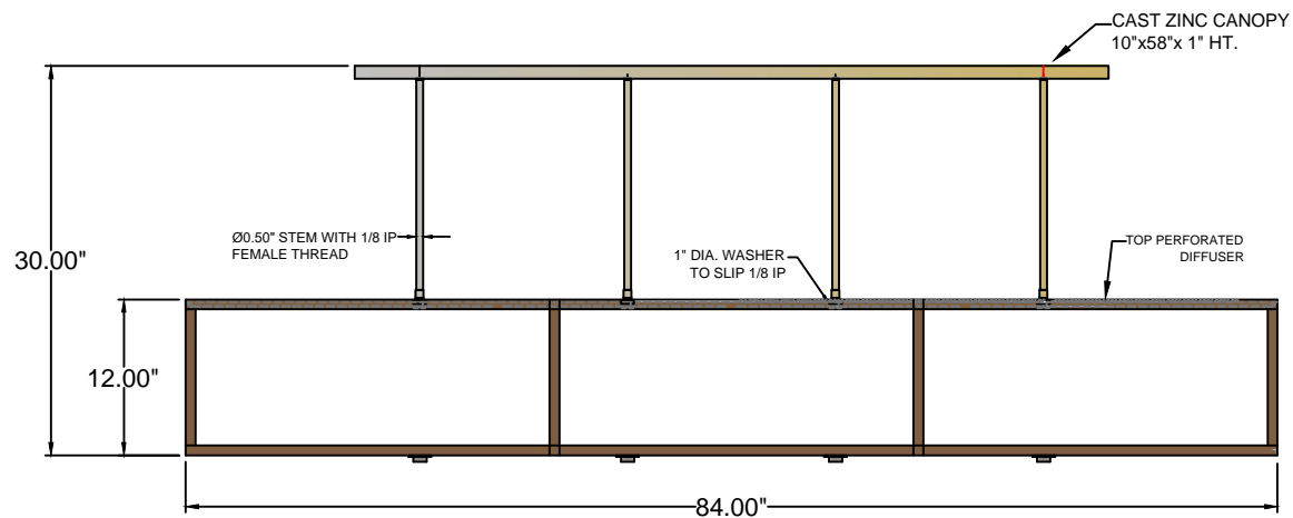
"FRONT VIEW "
