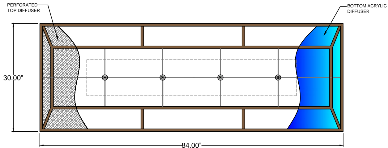
"BOTTOM VIEW "
